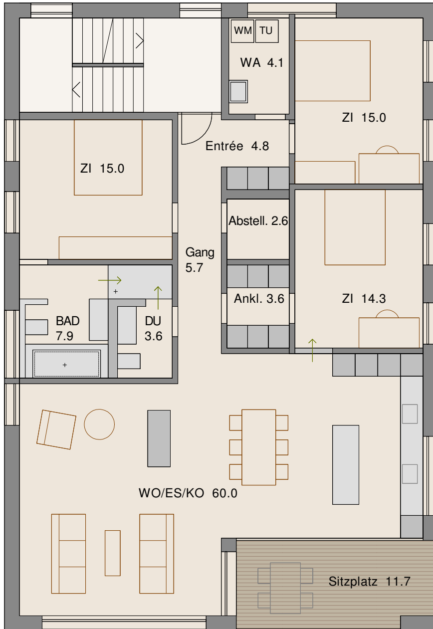
4 ½ Zi-Whg B 1.1 GF 162.0 m 2 / HNF 136.6 m 2
